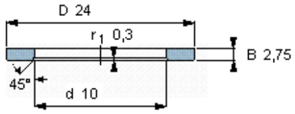
Universal washer
